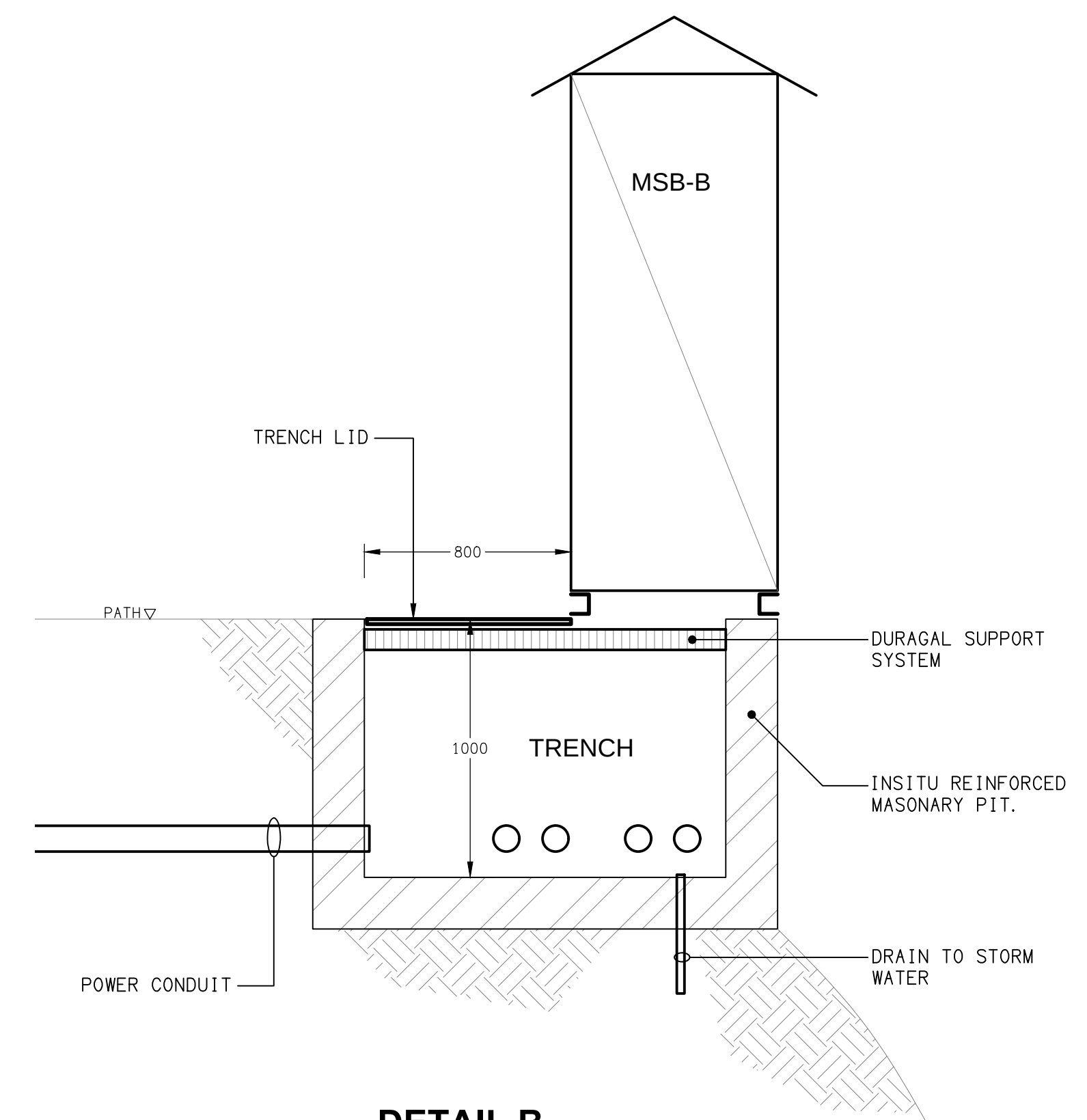
DETAIL B MSB-B & TRENCH SECTION SCALE 1: 20
