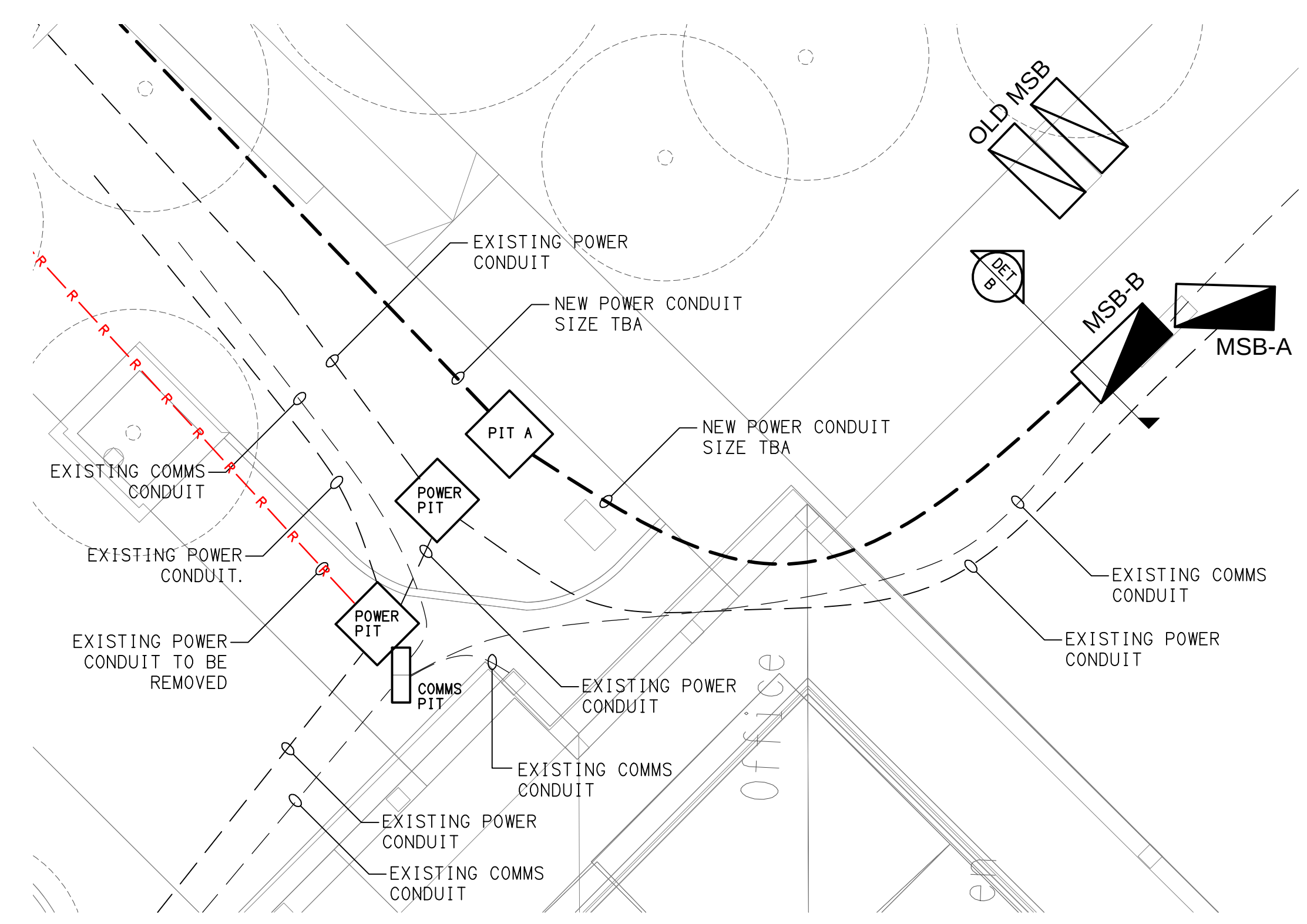
DETAIL A MSB & PIT PLAN SCALE 1: 100
